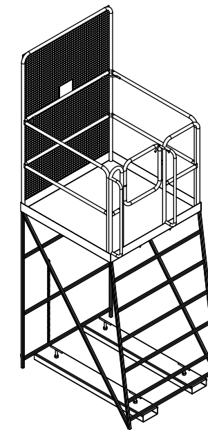
ISOMETRIC VIEW
