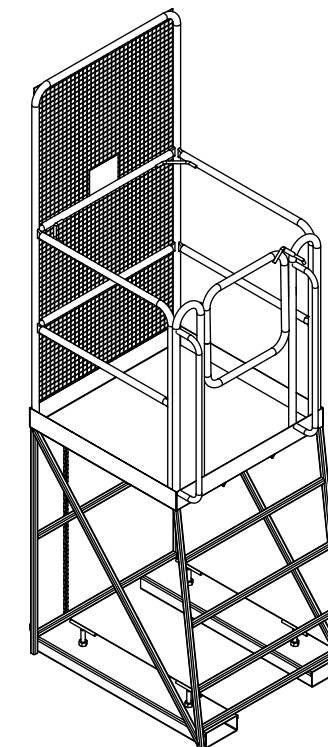
ISOMETRIC VIEW
