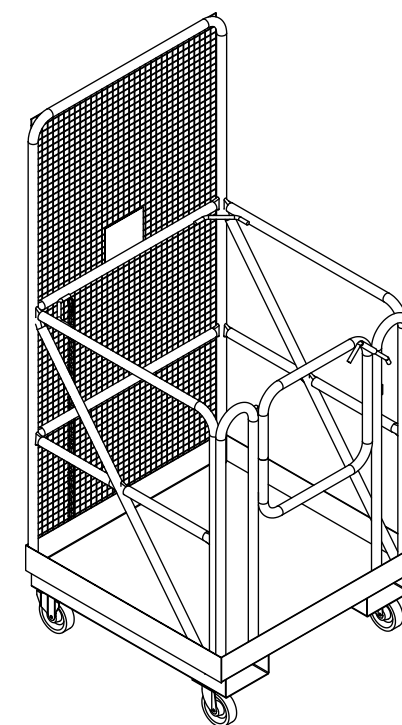
ISOMETRIC VIEW
