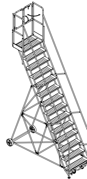
ISOMETRIC VIEW
