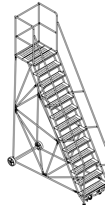
ISOMETRIC VIEW
