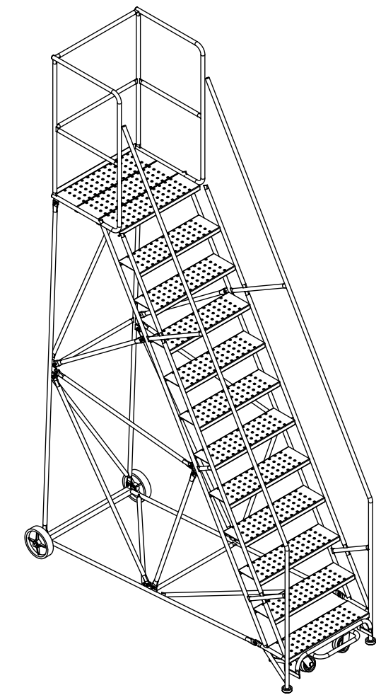
ISOMETRIC VIEW
