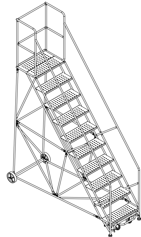
ISOMETRIC VIEW
