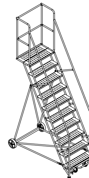
ISOMETRIC VIEW
