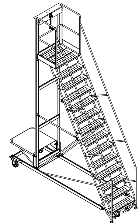
ISOMETRIC VIEW
